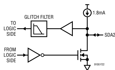
Figure 22. Isolated SDA2 Pin Schematic
