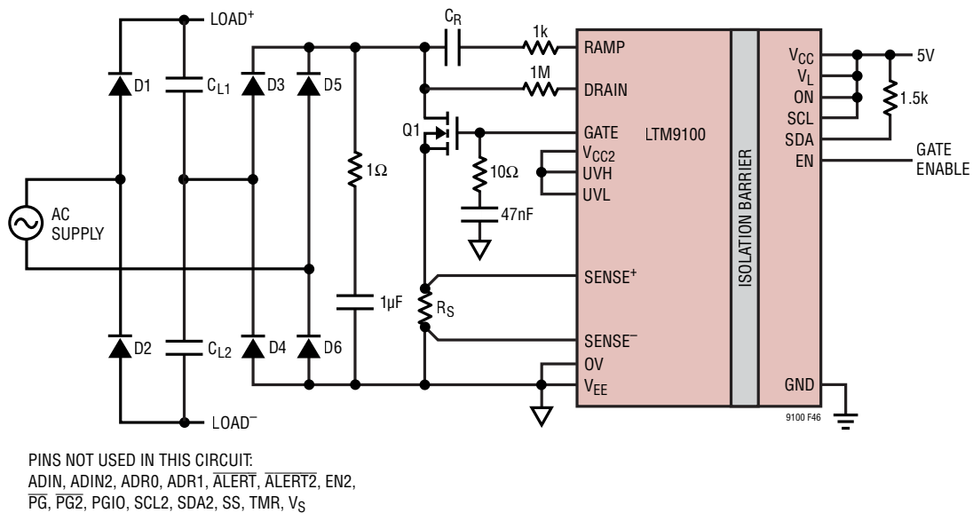
Figure 46. Inrush Current Limiting for AC Voltage Doubler
