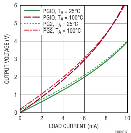
PG2, PGIO Output Low Voltage vs Load Current
