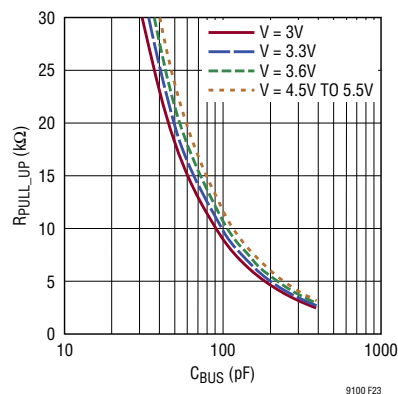
Figure 23. Maximum Standard Speed Pull-Up Resistance on SDA
