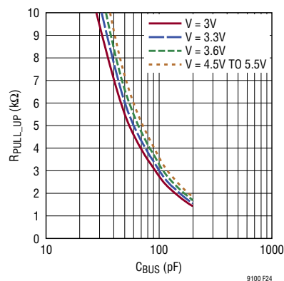
Figure 24. Maximum Fast Speed Pull-Up Resistance on SDA
